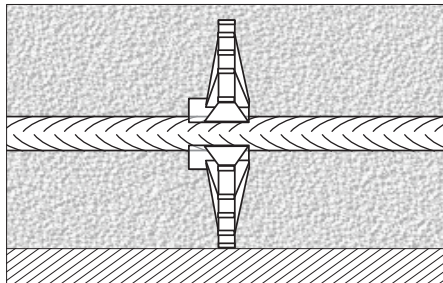
Plastic Wheels (clip-on)
